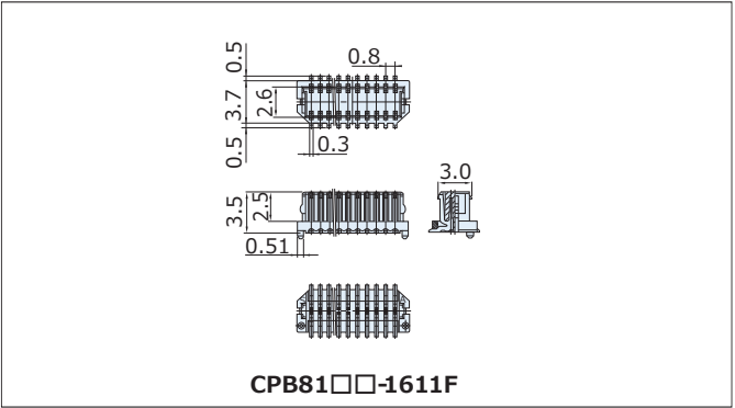
Plug (Straight Type) CPB82□□-☒☒11F
