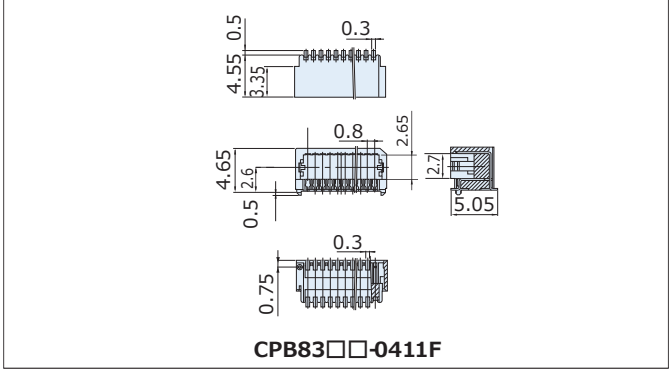
Plug (Right-Angle Type) CPB83□□-☒☒11F
