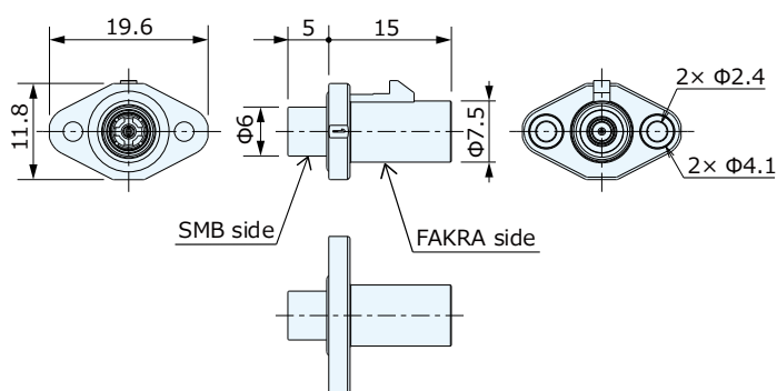
変換アダプタ：CKV9001-01□□F
