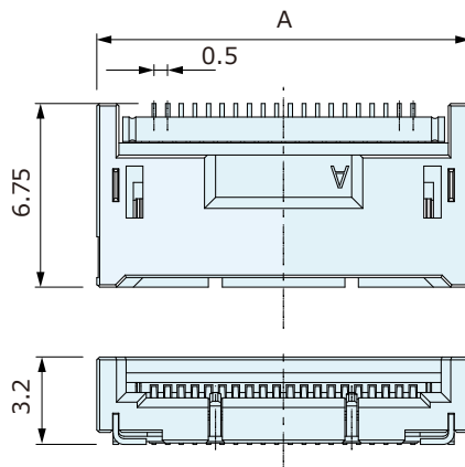
垂直型: CFPC725-0101F
