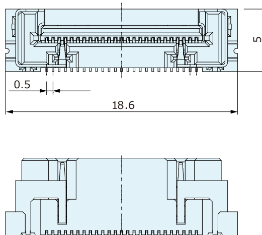
垂直型: CFPC725-0101F
