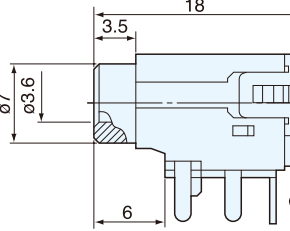
DIP Type
