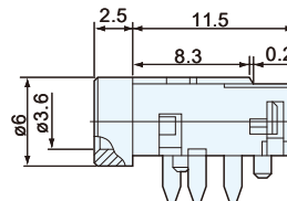
DIP Type
