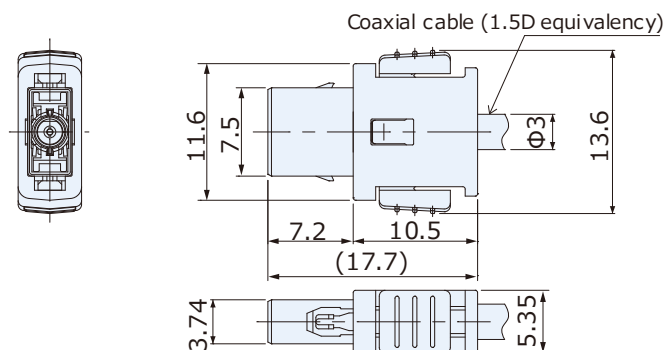
Plug: CRC9001-7701F
