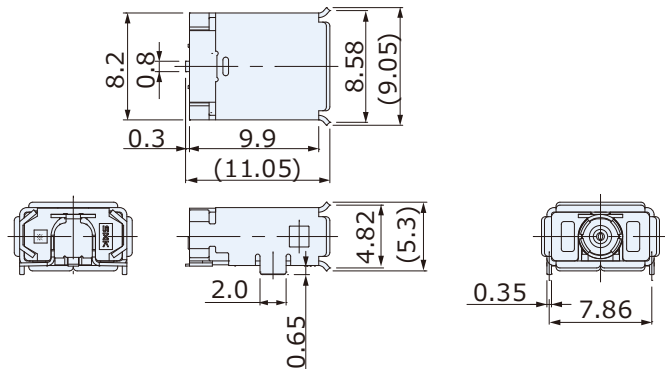
Receptacle: CRS5001-4701F
