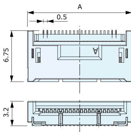
Right Angle Type : CFPC5□□-0101F
