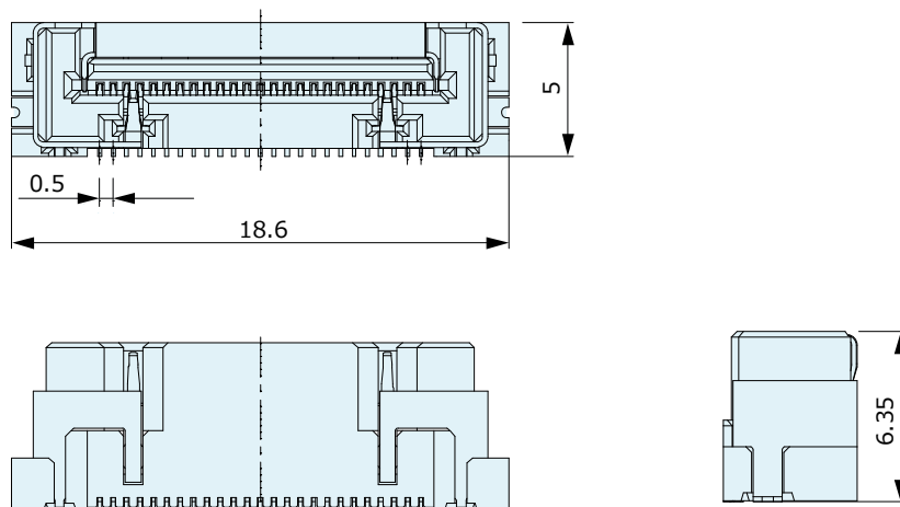
Vertical Type : CFPC725-0101F
